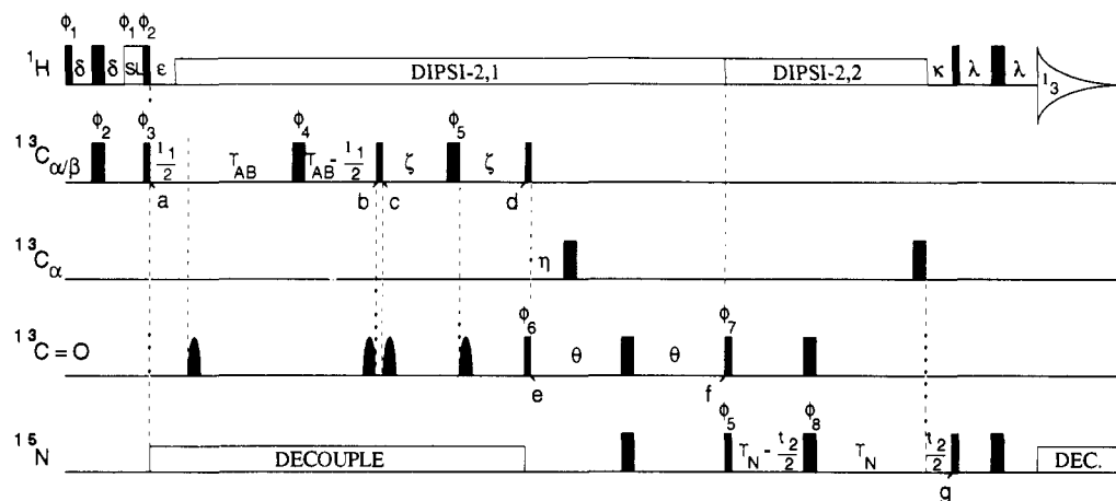
Figure 1. Pulse scheme of the CBCA(CO)NH experiment. Narrow pulses correspond to a 90^\circ flip angle and wider pulses to 180^\circ . Pulses for which no phase is indicated are applied along the x axis. The ^1\text{H} carrier is placed at 4.75 ppm until the 90_{\phi_7} CO pulse is applied. After this time the ^1\text{H} carrier is switched to 8.1 ppm. The C_{\alpha/\beta} carrier is positioned at 46 ppm and the power of the RF pulses is adjusted to yield zero excitation in the CO region (11.4-kHz RF for the 180^\circ and 5.1-kHz RF for the 90^\circ pulses at 151-MHz ^{13}\text{C} frequency). C_\alpha pulses are applied at 56 ppm, using an RF field of 10.5 kHz. Rounded carbonyl pulses have a 180^\circ flip angle and have the shape of the center lobe of a \sin x/x function and a duration of 202 \mu\text{s} . The second and third shaped CO pulses serve to compensate the C_{\alpha/\beta} phase errors caused by Bloch-Siegert effects 10 related to the first and fourth shaped pulse (see text). The rectangular CO pulses are applied using an RF field strength of 4.7 kHz, yielding minimal excitation of the C_\alpha resonances. All ^{15}\text{N} pulses are applied with the carrier at 117 ppm, using a 6-kHz RF field. ^{15}\text{N} decoupling was accomplished using low power (1.5-kHz RF) WALTZ decoupling. ^1\text{H} decoupling during the magnetization relay is accomplished with a DIPSI-2 scheme, 18 using a 5.5-kHz RF field. Delay durations are \delta = 1.5 ms, \epsilon = 2.3 ms, T_{AB} = 3.3 ms, \eta = 4.5 ms, \theta = 11.4 ms, T_N = 11.1 ms, \kappa = 5.4 ms, \lambda = 2.25 ms. The \text{H}_2\text{O} resonance was suppressed with the 1.8-ms purge pulse, SL. Phase cycling was as follows: \phi_1 = y ; \phi_2 = x, -x ; \phi_3 = x ; \phi_4 = 8(x), 8(y), 8(-x), 8(-y) ; \phi_5 = 4(x), 4(-x) ; \phi_6 = 2(x), 2(-x) ; \phi_7 = 51^\circ (Bloch-Siegert phase error compensation); \phi_8 = 8(x), 8(-x) ; Rec. = x, 2(-x), x, -x, 2(x), 2(-x), 2(x), -x, x, 2(-x), x . Quadrature in F_1 and F_2 is obtained by altering \phi_3 and \phi_5 in the usual manner. 2
