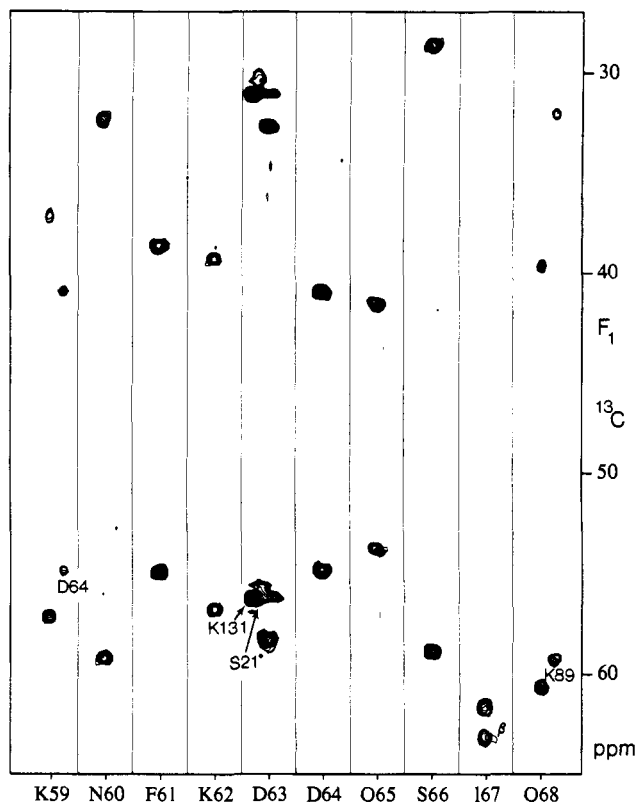
Figure 2. F_1 ( C_\alpha , C_\beta ) strips for residues K59–Q68, taken from the 600-MHz 3D CBCA(CO)NH spectrum of interferon- \gamma at the ^1\text{H}/^{15}\text{N} ( F_3/F_2 ) frequencies of their amides. In the leftmost strip, the amide of K59 correlates with C_\alpha and C_\beta of F58. Also visible in this strip is the correlation for the amide of D64 (which has a ^1\text{H} - ^{15}\text{N} correlation very close to that of K59) to the C_\alpha and C_\beta of D63. These latter correlations are observed with much higher intensity in the sixth strip.
